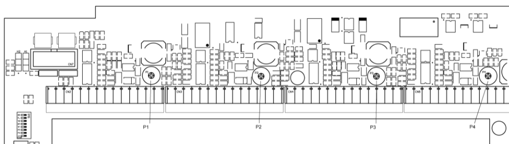
Back plane PCB PC-5120.
