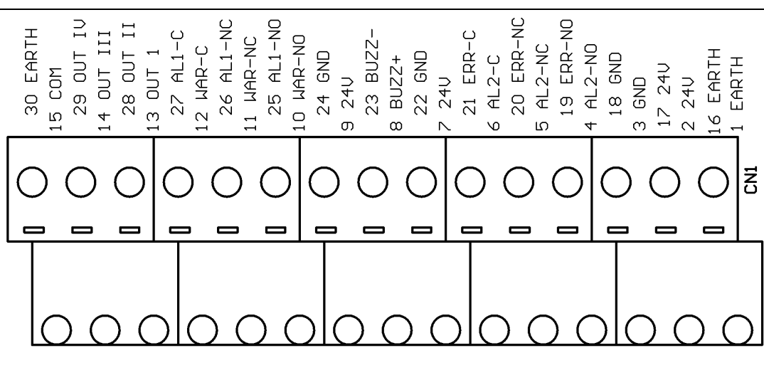
Internal terminal block.
